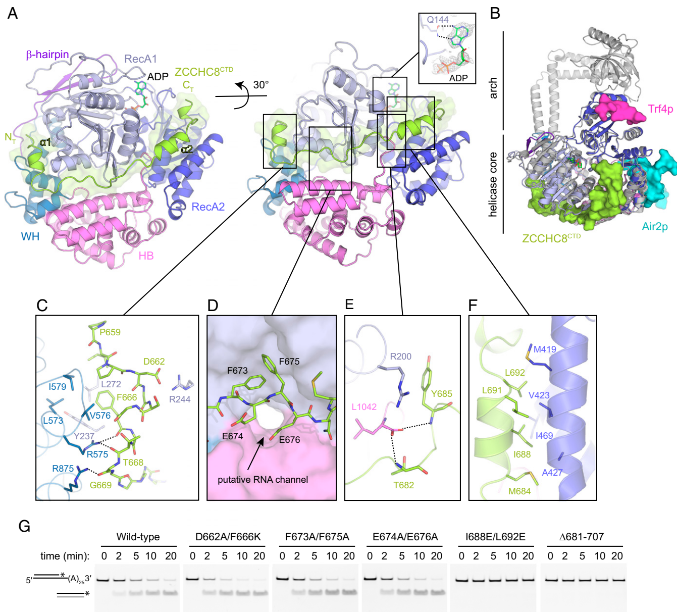
Fig. 6. Structure of the ZCCHC8 CTD -MTR4 ΔNA Arch complex. (A) Overall structure of ZCCHC8 CTD (lemon green) bound to the helicase core of MTR4. N T and C T denote the N and C termini of ZCCHC8 CTD . (Inset) A snapshot of a simulated annealing omit map (gray mesh) from the modeled ADP, contoured at 0.9 σ. (B) Superposition of ZCCHC8 CTD -MTR4 ΔNA Arch model (color scheme as in A) with the structure of S. cerevisiae Mtr4p (light gray) in complex with Trf4p (magenta) and Air2p (teal) peptides (PDB ID code 4U4C). (C–F) Magnified views of the interaction of the ZCCHC8 CTD peptide with MTR4. (G) Unwinding assays of NEXT reconstituted with the indicated ZCCHC8 variant. Reactions were performed using a 3' A 25 tailed duplex substrate and 500 nM protein. Assays were performed in triplicate with a representative gel for each sample shown.
