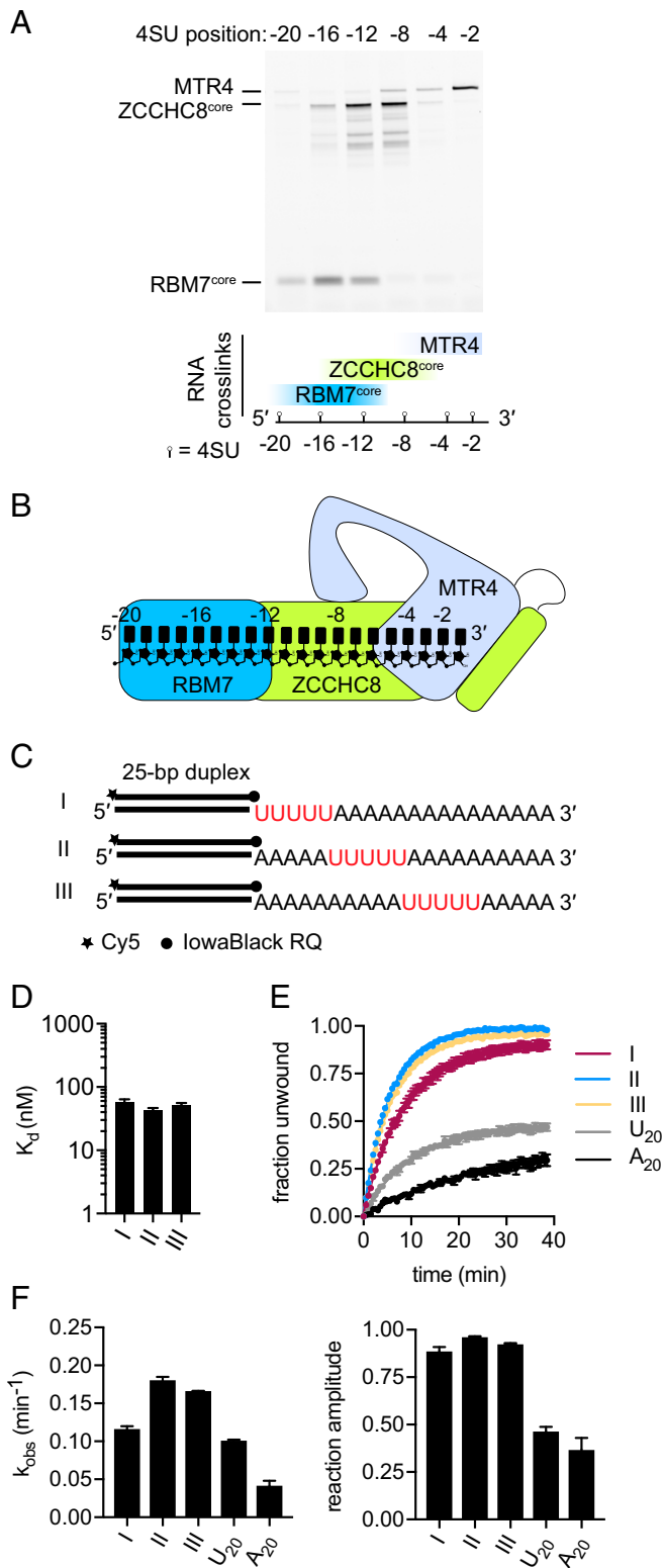
Fig. 4. Interaction of NEXT with RNA. (A) Site-directed 4-thiouridine crosslinking assay of NEXT with an A 20 substrate. (B) Diagram showing the proposed RNA binding path in NEXT. (C) Molecular beacon RNA duplex substrates I to III used to test the effect of the position of uridine sequences on RNA affinity and helicase activity of NEXT. (D) Bar graph showing the equilibrium dissociation constant ( K_d ) of NEXT on substrates I to III. Dissociation constants were measured using EMSA. Error bars represent \pm SD from three experiments ( n = 3 ). (E) Molecular beacon helicase assay of NEXT. (F) Bar graph showing the observed rate constants and reaction amplitudes obtained for substrates I to III, 3' A 20 tailed duplex, and 3' U 20 tailed duplex. Error bars represent \pm SD.
